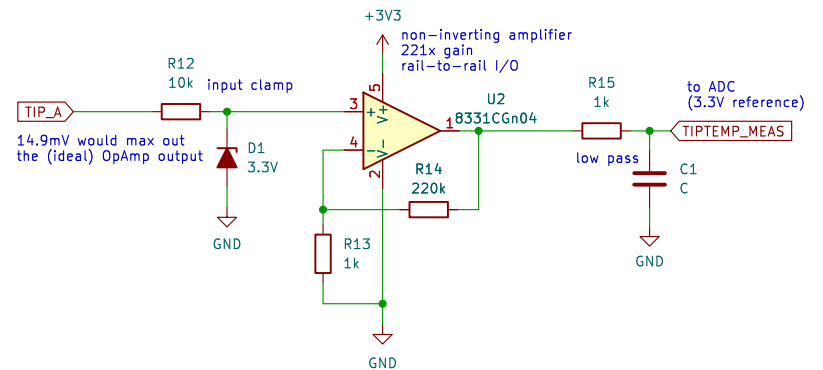
T12 soldering tip temperature measurement
