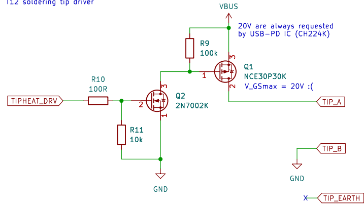
T12 soldering tip driver
